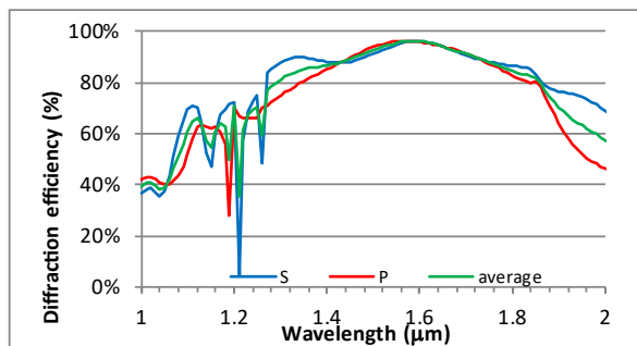
Typical absolute diffraction efficiency at AOI 47.5° *
