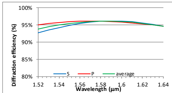
Typical absolute diffraction efficiency at AOI 47.5° *
