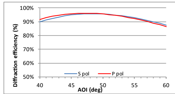
Diffraction efficiency at 1568 nm as a function of AOI *
