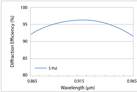
Typical absolute diffraction efficiency at AOI 57.9°*
