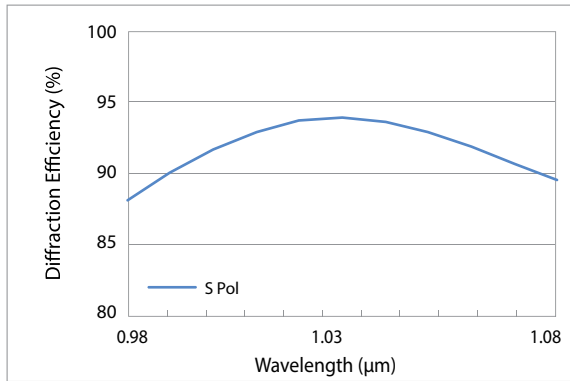
Typical absolute diffraction efficiency at AOI 63.6°*
