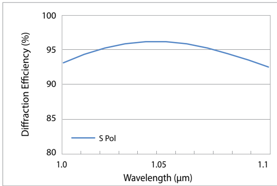
Typical absolute diffraction efficiency at AOI 55.5°*
