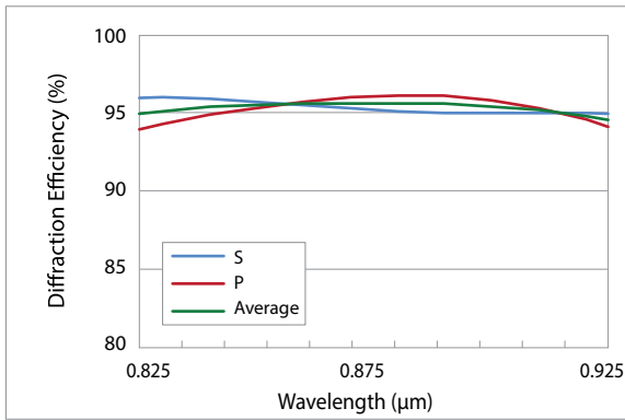
Typical absolute diffraction efficiency at AOI 41.1°*
