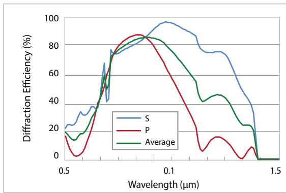
Typical absolute diffraction efficiency at AOI 50.9° *
